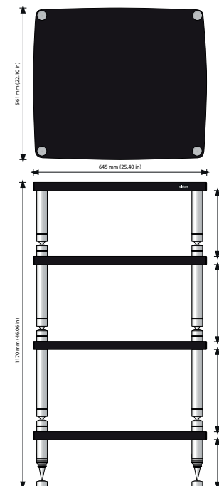
HF-4 COLOSSUS SPECIAL HYPERSPIKE HIGH-END AUDIO RACK
